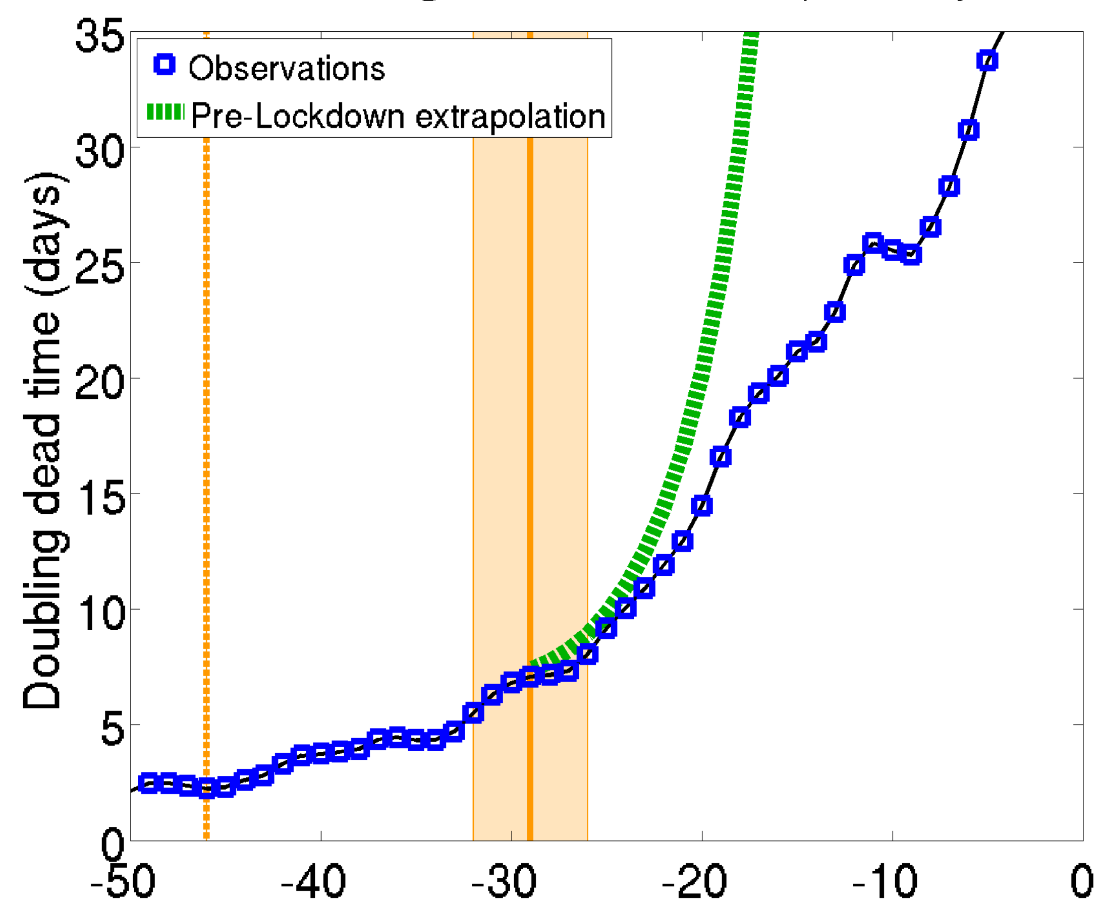
Time of doubling total dead number | Country : ITA
