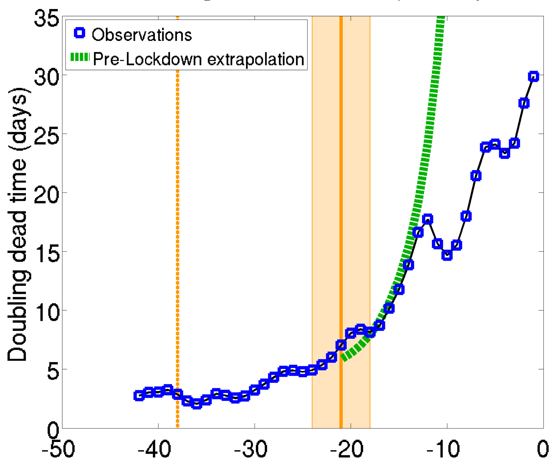
Time of doubling total dead number | Country : FRA
