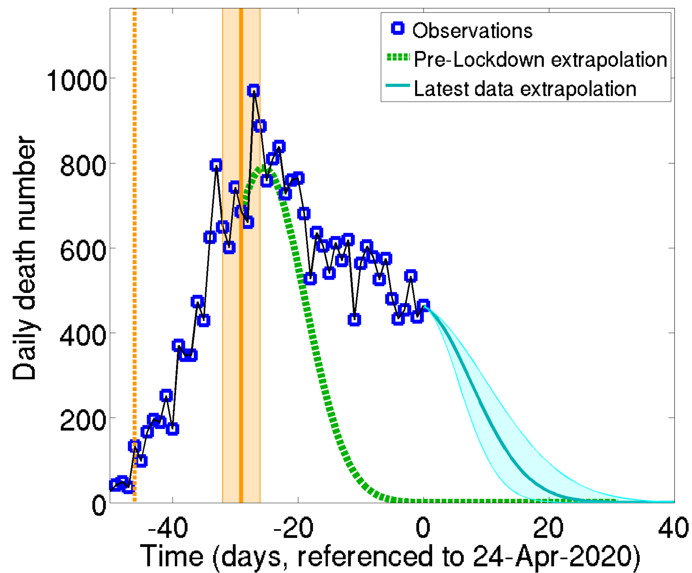
Daily death number | Country : GBR
