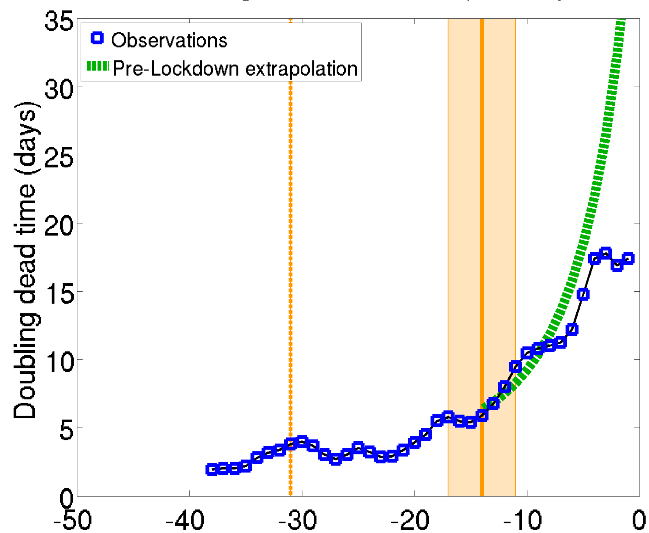
Time of doubling total dead number | Country : GBR
