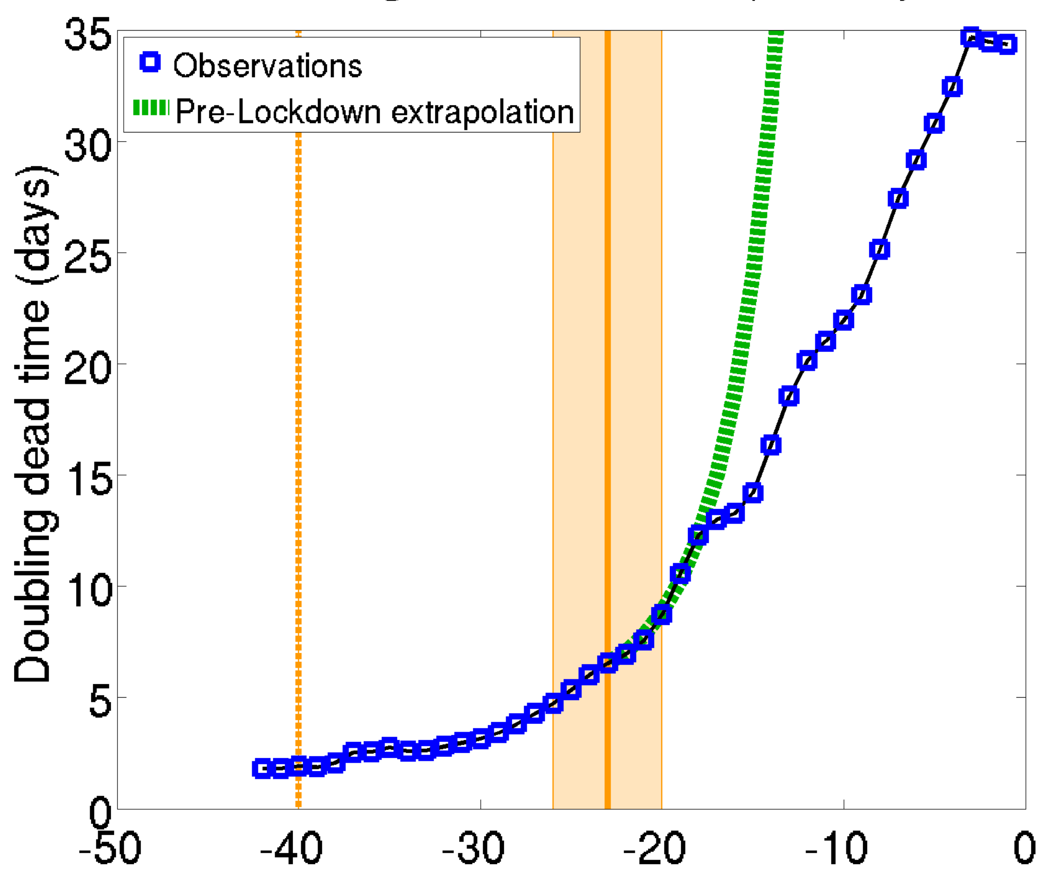
Time of doubling total dead number | Country : ESP
